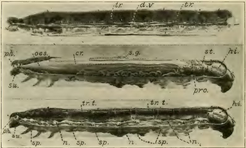
FIG. 23.—Internal anatomy of silk-worm, from photo of Azoux Model: A, upper or dorsal bodywall seen from within; B, the back of the silk-worm removed, showing alimentary canal; C, alimentary canal removed, showing nervous system and tracheal trunks; tr. , trachea; d.v. , dorsal vessel or heart; ph. , pharynx or mouth; su. , supra-oesophageal ganglion; sp.sp. , spiracles or breathing pores; n. , nerve cord; tr.t. , tracheal trunk; oes. , oesophagus or throat; cr. , crop; s.g. , silk gland; pro. , proventriculus; st. , stomach; h.i. , hind intestine.
